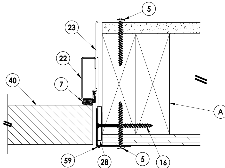
4 HORIZONTAL CROSS SECTION 2x Stud Construction Outswing Shown (Inswing Similar)
