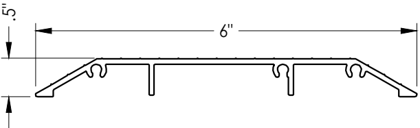
31 ADA THRESHOLD AFCO A-202
