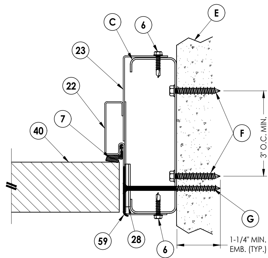
2 HORIZONTAL CROSS SECTION 4 Steel Stud Construction Outswing Shown (Inswing Similar)
