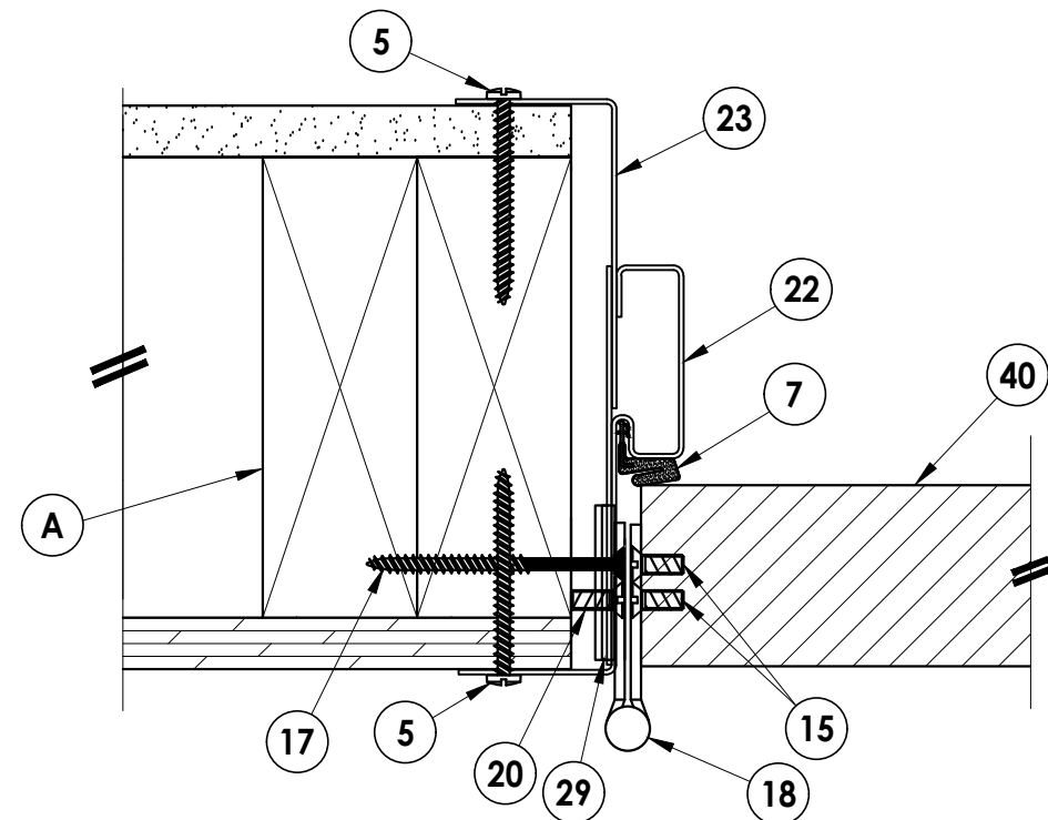
3 HORIZONTAL CROSS SECTION 4 2x Stud Construction Outswing Shown (Inswing Similar)
